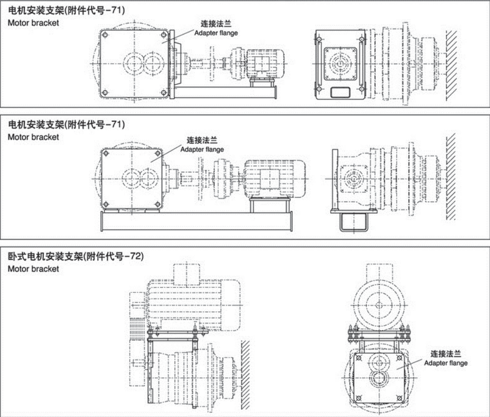
法兰联接及底座安装时螺母的预紧扭矩: Tightening Torques for Flange Connections and Foot-mounted Design:
